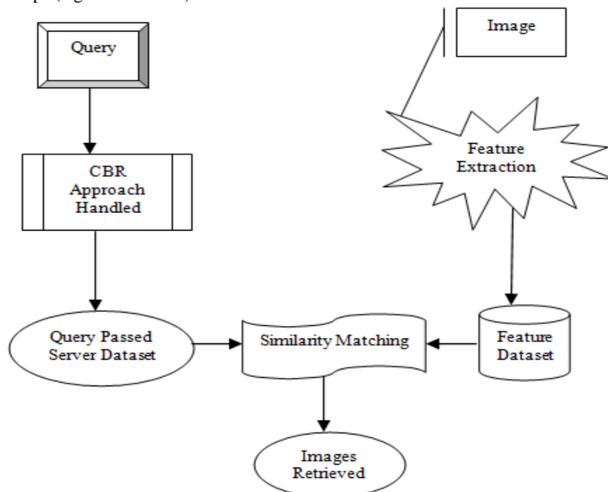
Fig. 2: System Architecture
