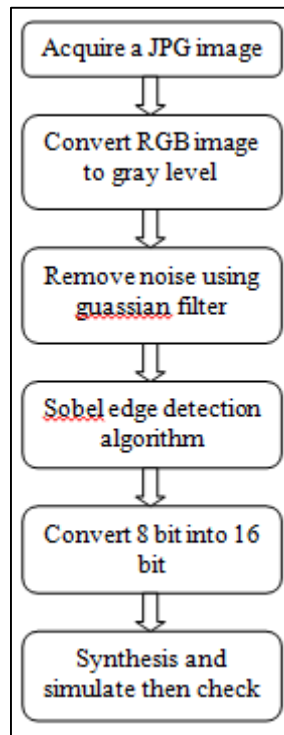
Fig. 1: Proposed flow chart
