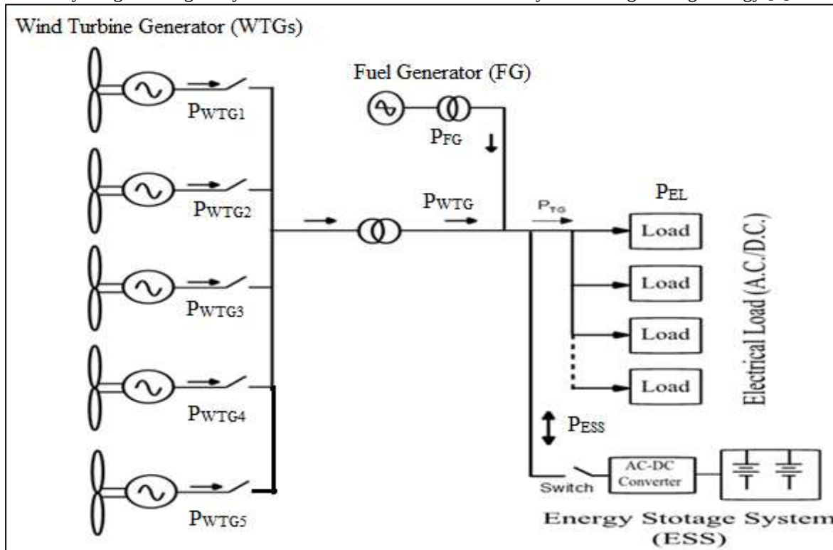
Fig. 1: Block Diagram of system developed diagram
