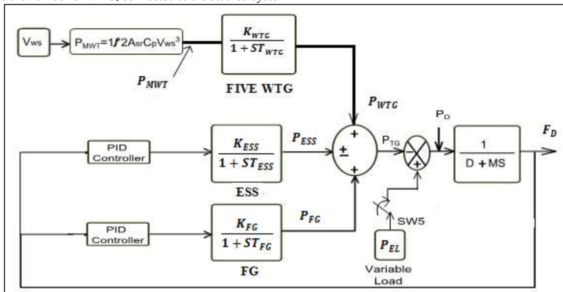
Fig. 3: Block Diagram of CASE-II
