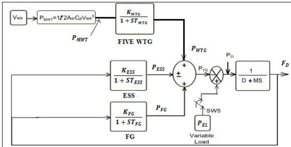
Fig. 2: Block Diagram of CASE-I
