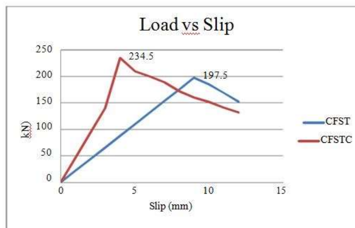
Fig. 6: Failure load
