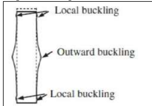
Fig. 9: Failure Pattern
