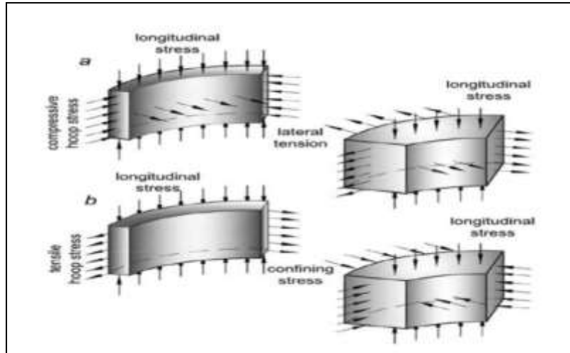
Fig. 1: Stress condition in steel tube and concrete core at different stages of loading
