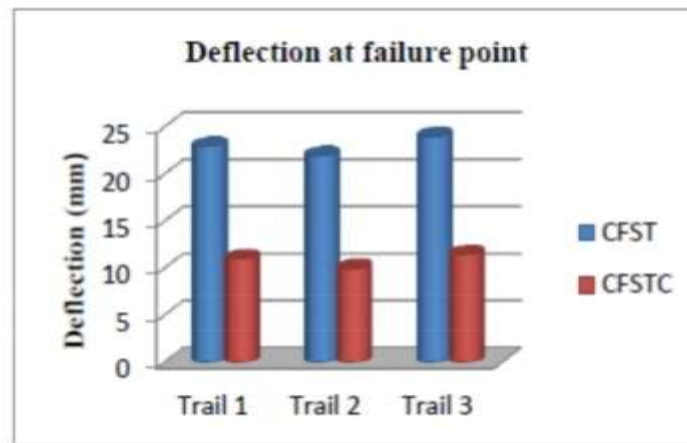
Fig. 8: Deflection at Failure load
