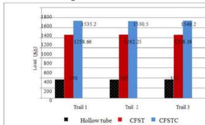
Fig. 7: Comparison of failure loads
