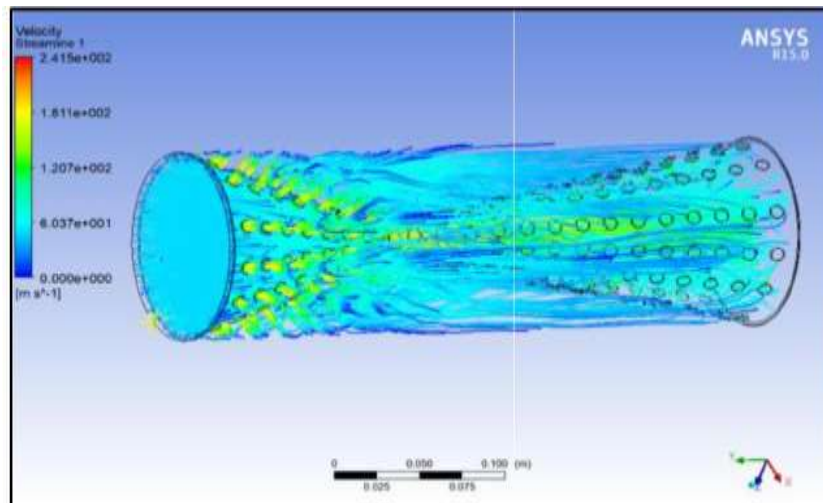
Fig. 4: Distribution of velocity streamlines through the ducts
