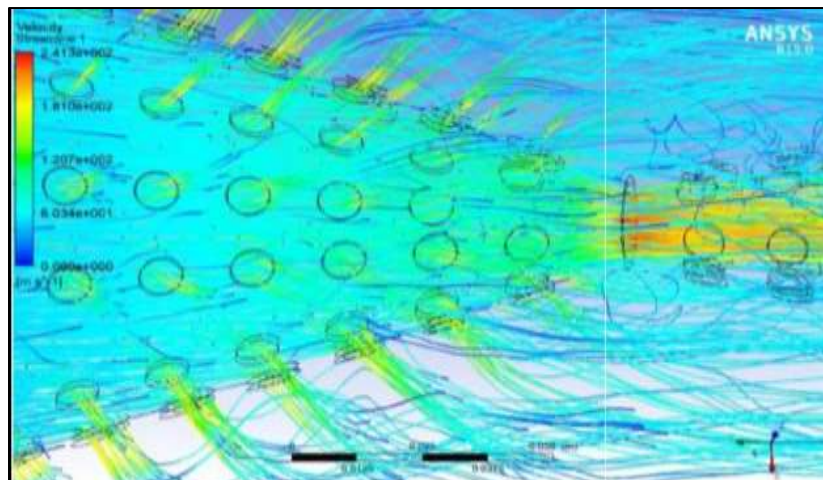
Fig. 5: Figure showing velocity of scattered exhaust particles through the ducts
