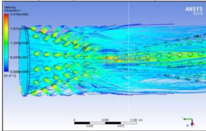
Fig. 3: Velocity distribution of exhaust gases in the muffler
