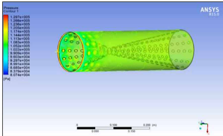
Fig. 6: Pressure contour 1
