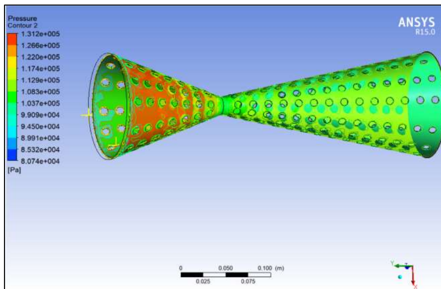
Fig. 7: Pressure contour 2
